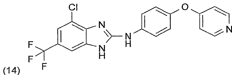
(4-Chloro-6-trifluoromethyl-1H-benzimidazol-2-yl)-[4-(pyridin-4-yloxy)-phenyl]-amin
